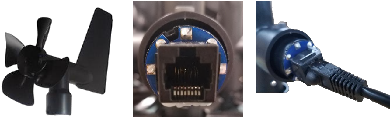
Figure 12: Miniaervane connections
