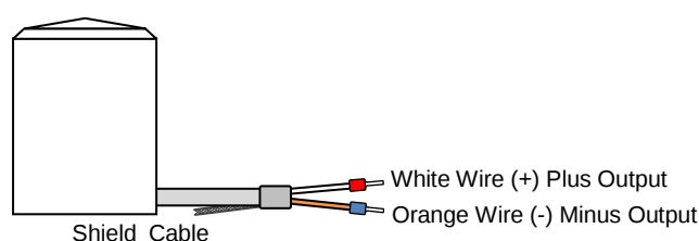
Figure 7-1. Signal cable
