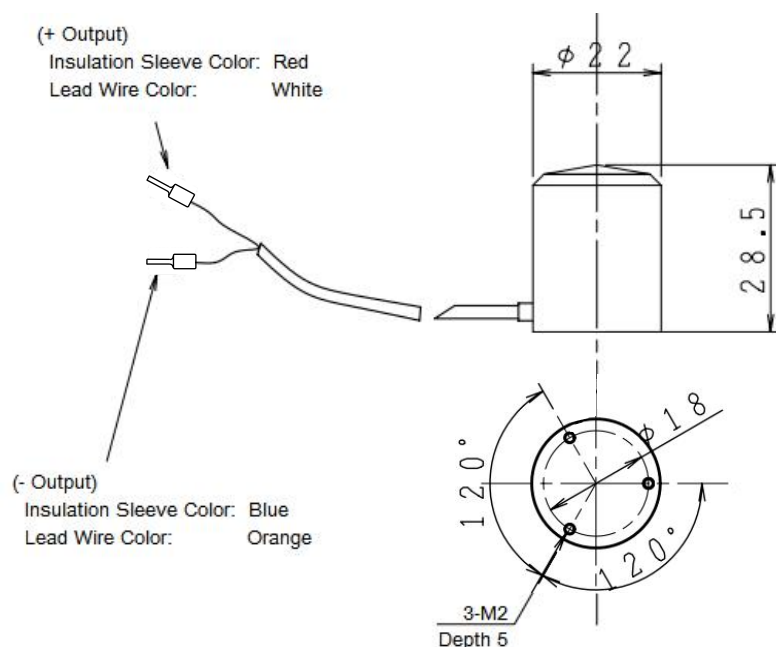
Figure 7-2. Outer Dimensions of Sensor
