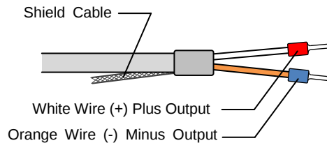
Figure 5-4. Signal cable Ends Polarity
