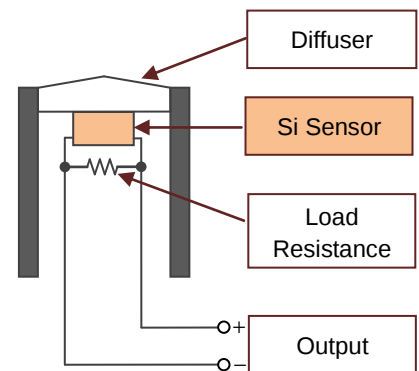
Figure 5-5. ML-01 Construction
